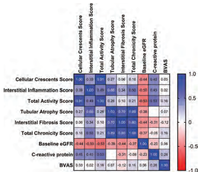
Figure 1. Variables correlation.
