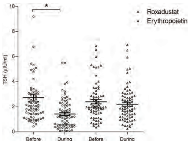
TSH change
