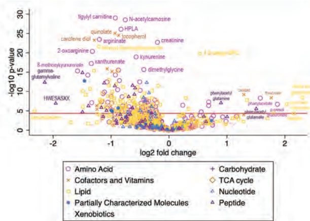
Volcano Plot
