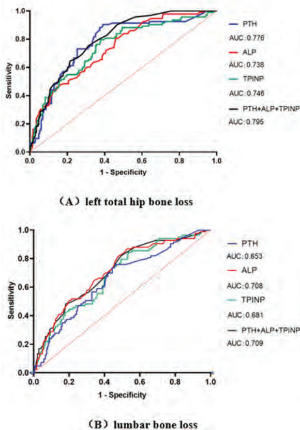
Figure 2 ROC curve
