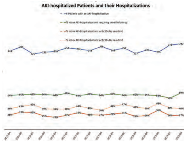
Fig 1. Quarterly trends
