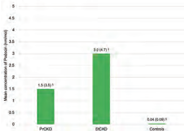
Figure 1, Podocin Concentrations
