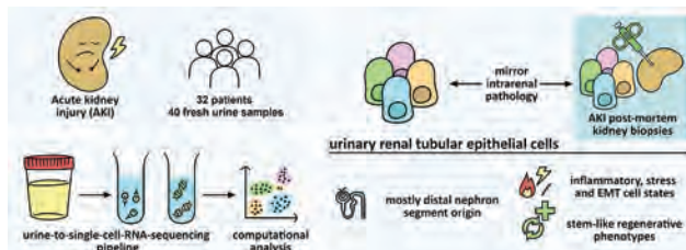
Graphical abstract
