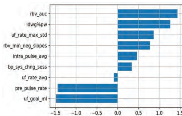
Figure 1. Feature list
